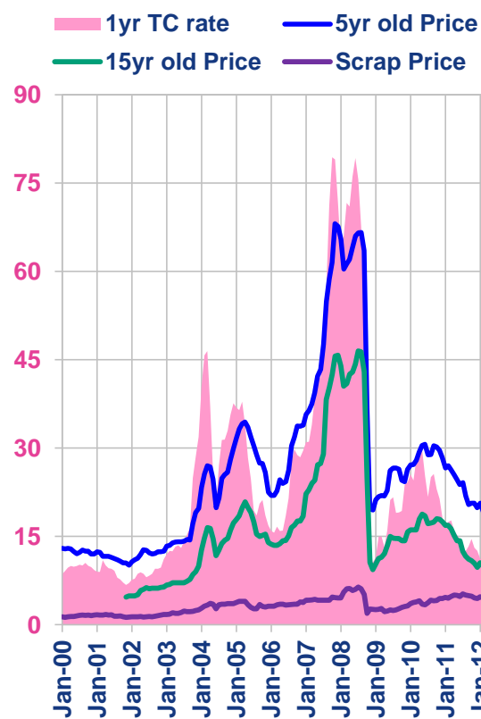
P'max Bulker
