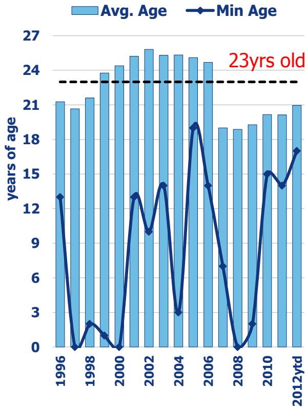
Crude Tanker
